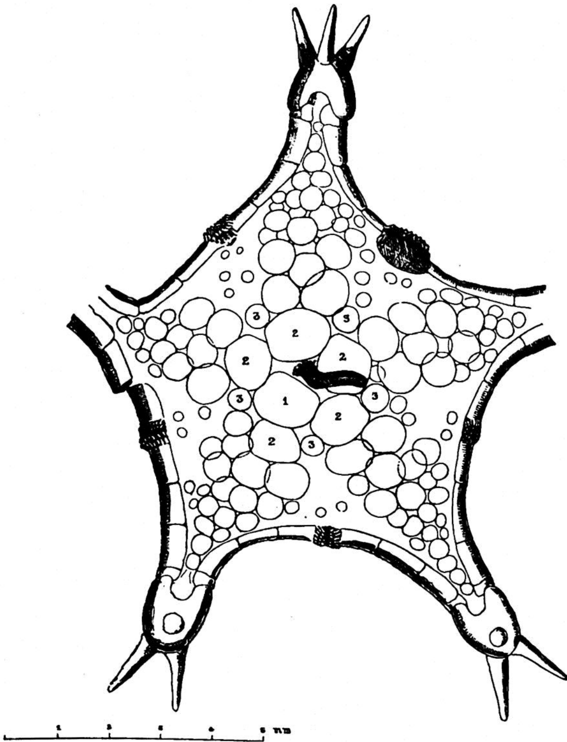
Porcellanaster eremicus , n. sp. Outline sketch of a young example, to show the abactinal plating. Magnified 13 diameters. The following primary apical plates are indicated by numbers:—1. Dorsal-central; 2, 2. Under-basals; 3, 3. Basals.
