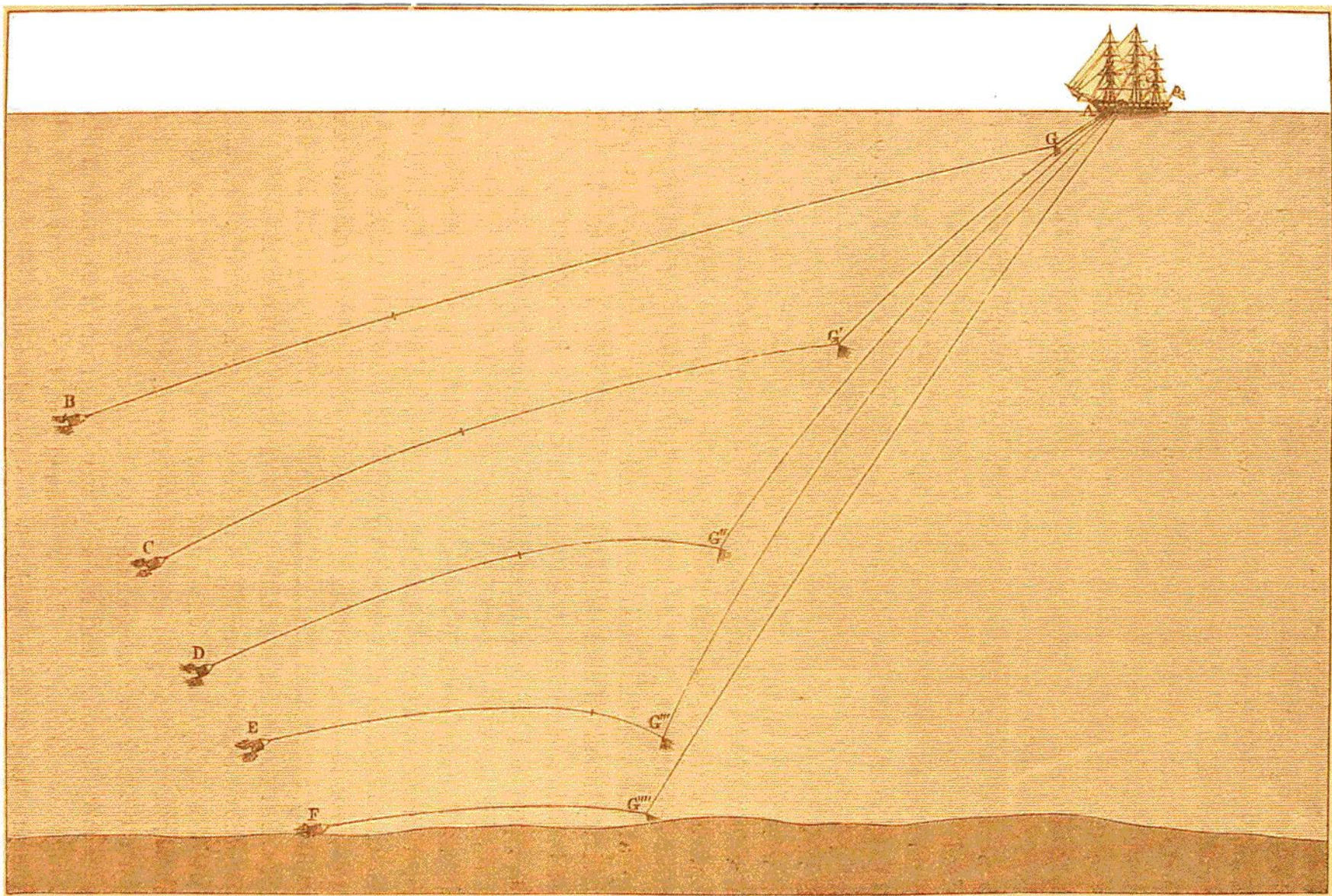
FIG. 10.—The relative positions of the Ship, the "Messenger" Weights, the "Toggle" and the Dredge, at different stages of "Paying out" from the CHALLENGER.
