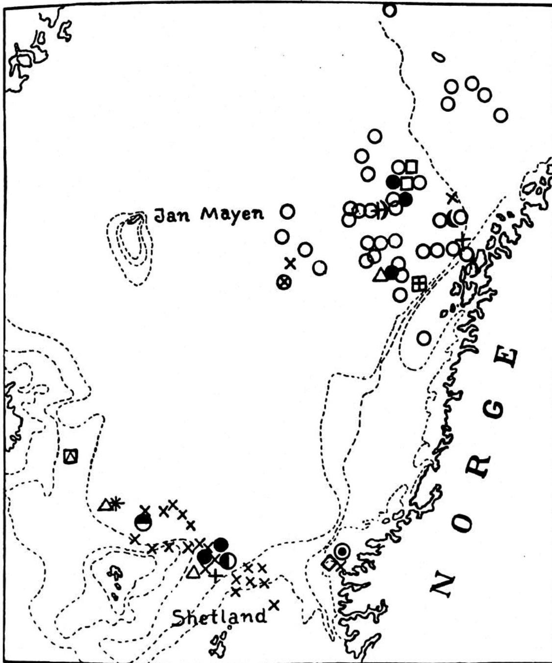
FIG. 482.—ANIMALS CAUGHT OVER GREAT DEPTHS IN THE NORWEGIAN SEA. The isobaths represent depths of 100, 200, and 500 fathoms.
