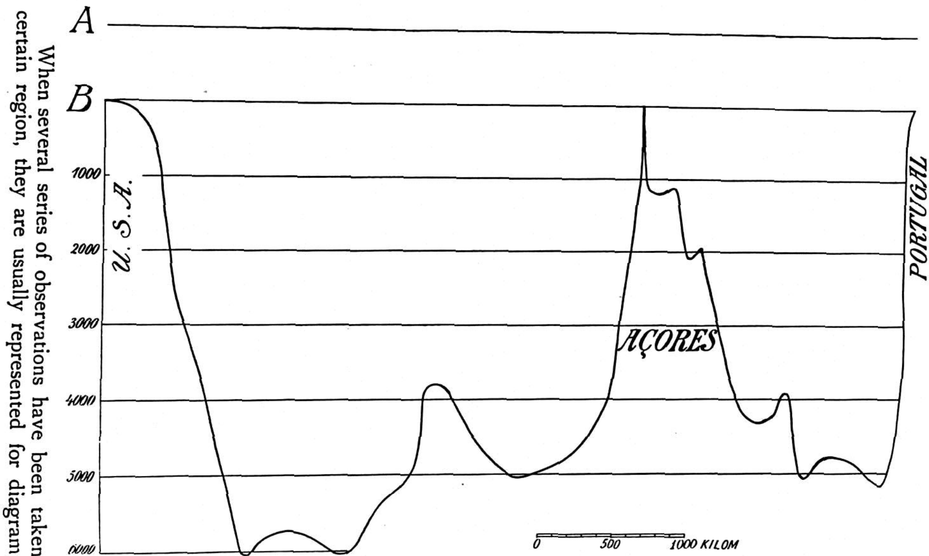
FIG. 152.—SECTION SHOWING THE FORM OF THE BOTTOM OF THE ATLANTIC OCEAN ALONG THE PARALLEL OF 40^{\circ} N. B shows the vertical scale exaggerated 500 times as compared with the horizontal. On the natural scale the section looks like a straight line ( A ).
