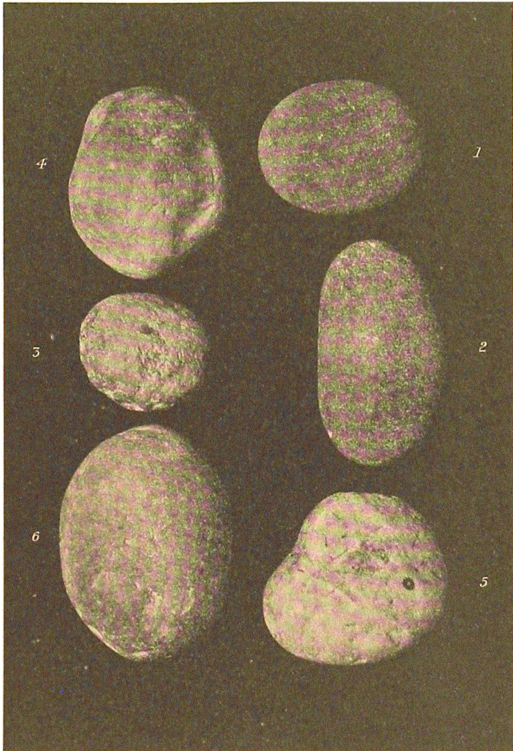
FIG. 146.—ROUNDED STONES FROM "MICHAEL SARS" STATION 95.
