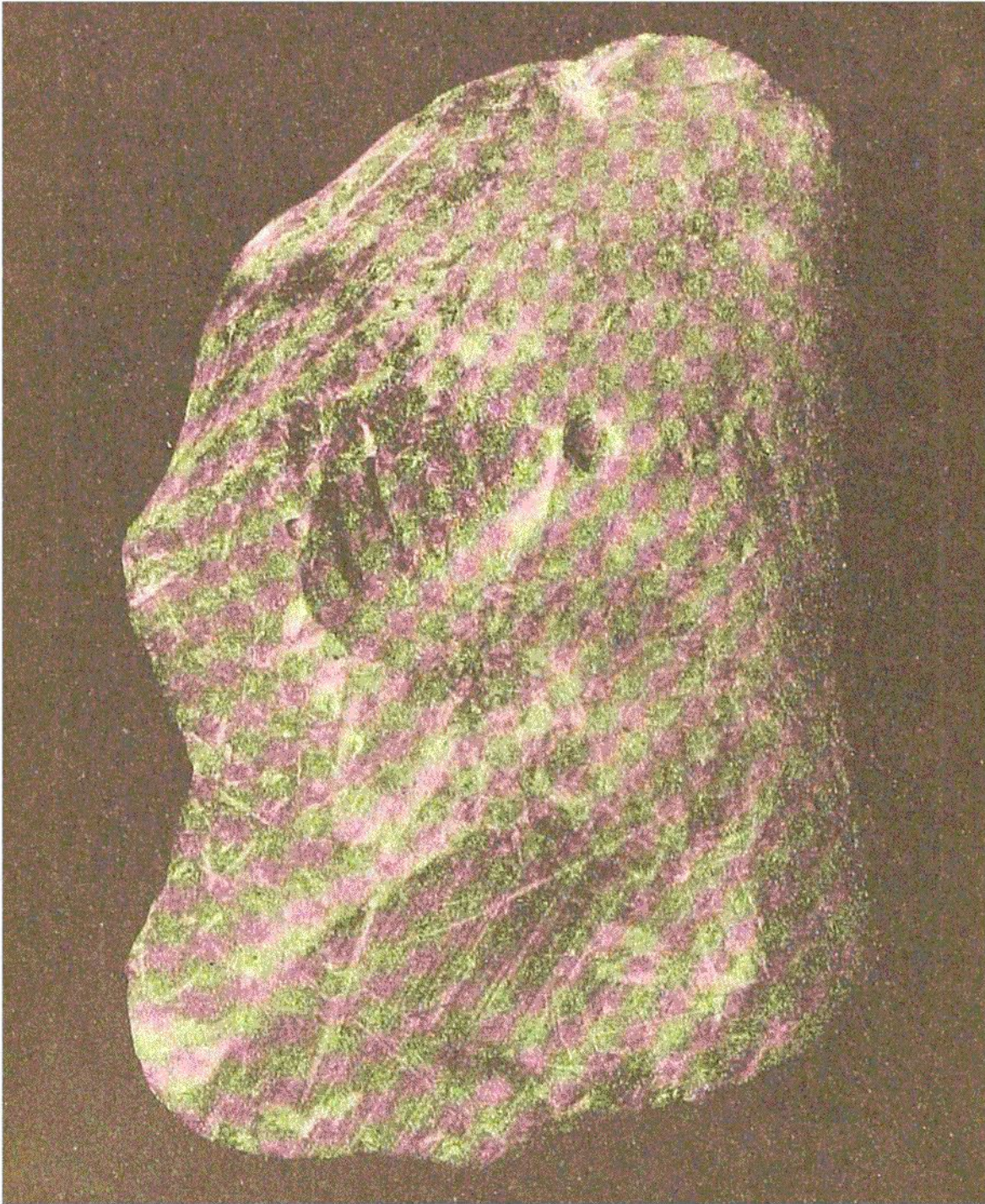
FIG. 145.—GLACIATED STONE FROM "MICHAEL SARS" STATION 95.
