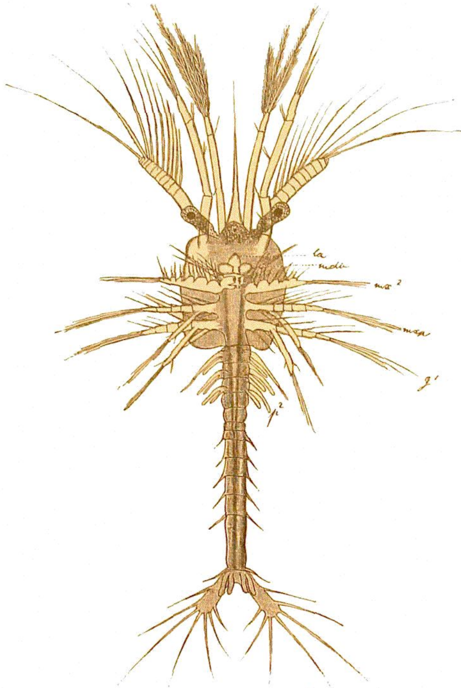
FIG. 44 (D).—Zoea of Sergestes tenuis (?). From a drawing by Dr. v. Willemoes-Suhm. p^2 , three pairs of pereiopoda. Other lettering as before.
