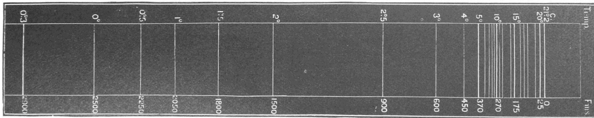
FIG. 56.—Diagram of the Vertical Distribution of Temperature at Station CCCXXVII.
