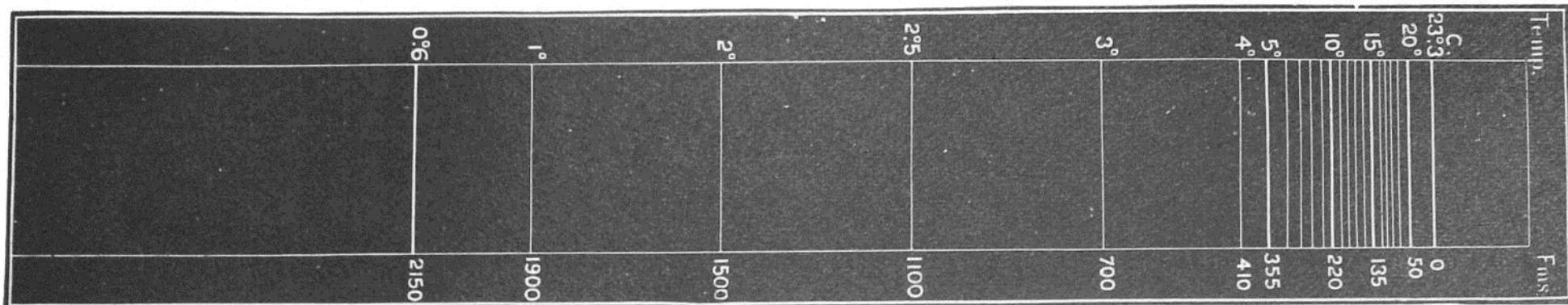
FIG. 55.—Diagram of the Vertical Distribution of Temperature at Station CXXIX.
