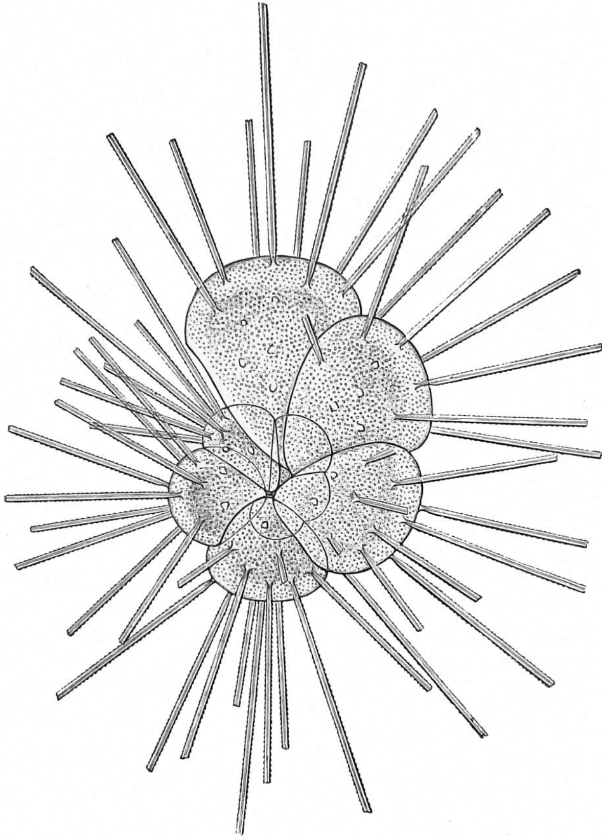
FIG. 51. — Hastigerina Murrayi , WYVILLE THOMSON. From the surface. Fifty times the natural size.
