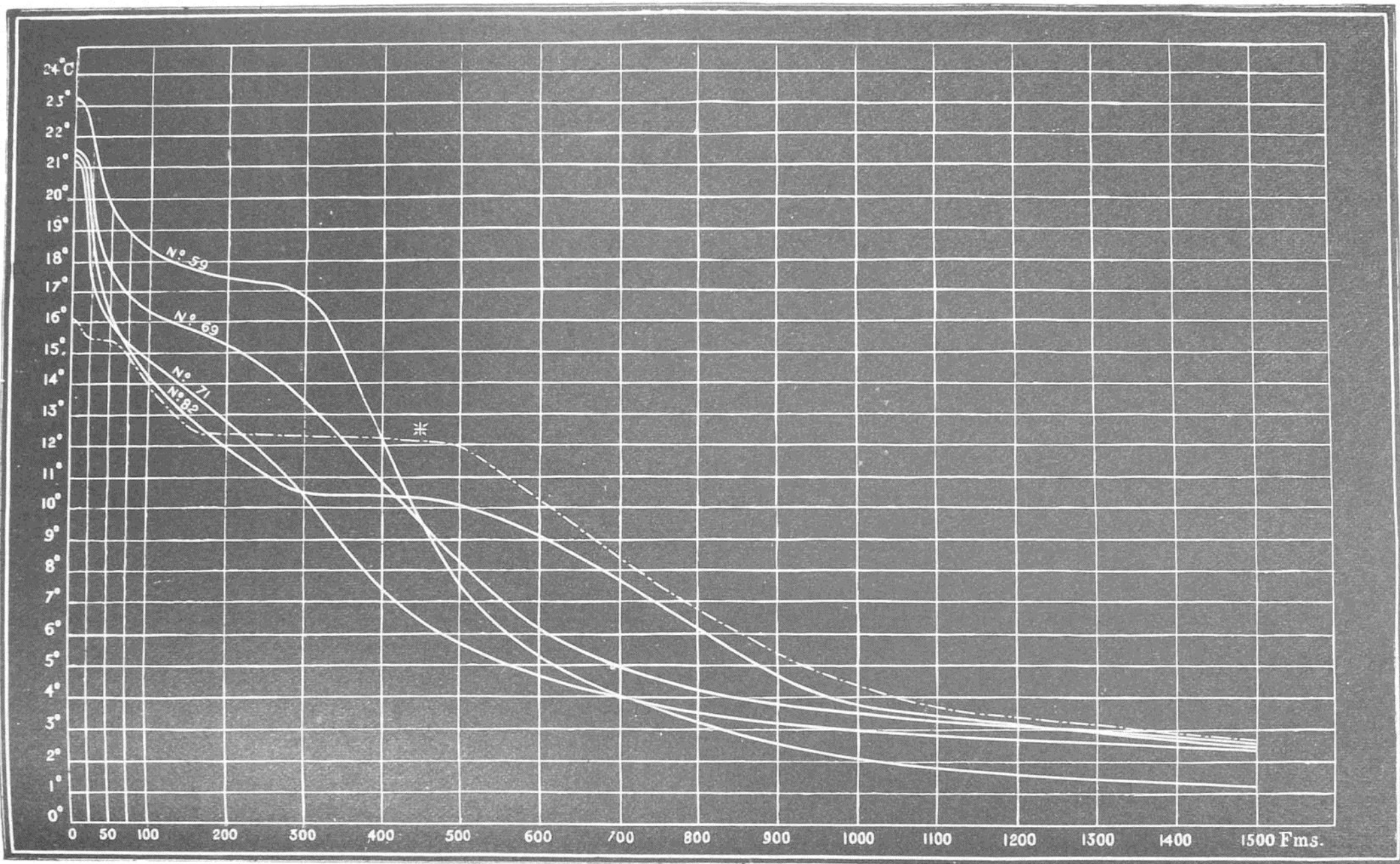
FIG. 13.—Curves constructed from the Serial Soundings at Stations LIX., LXIX., LXXI., and LXXXII. The dotted line representing the temperatures taken in 1869-70 off the coast of Portugal is introduced for comparison.
