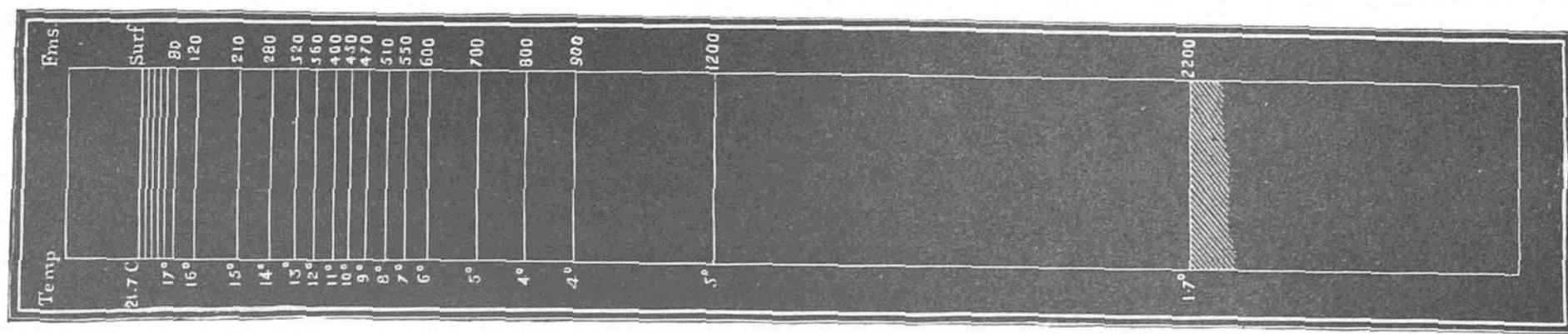
FIG. 5.—Diagram showing the Relation between Depth and Temperature at Station LXXI.
