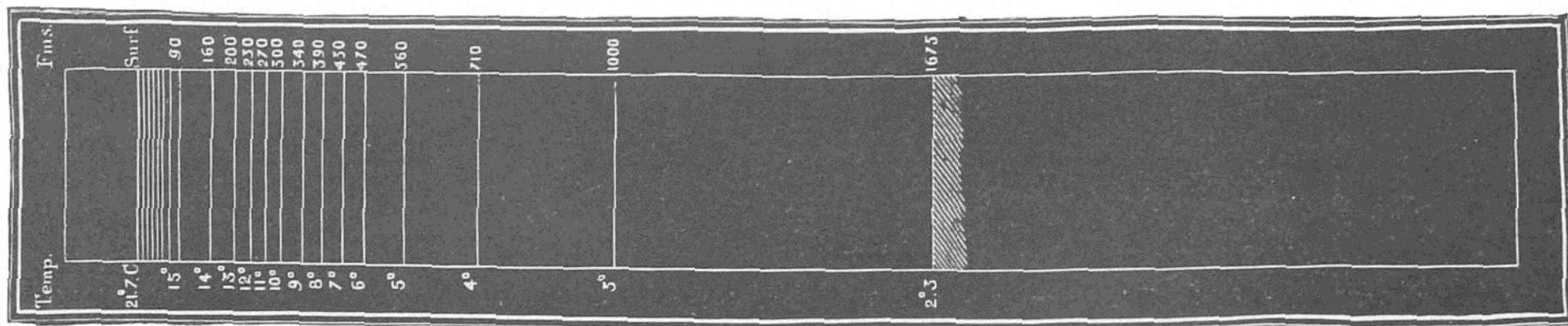
FIG. 4.—Diagram showing the Relation between Depth and Temperature at Station LXIX.
