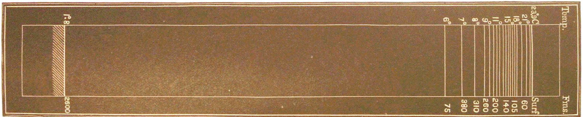
FIG. 92.—Diagram showing the Relation between Depth and Temperature at Station XLIII.
