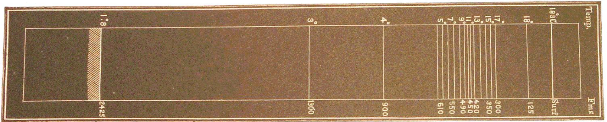
FIG. 91.—Diagram showing the Relation between Depth and Temperature at Stations XLI. and XLII.
