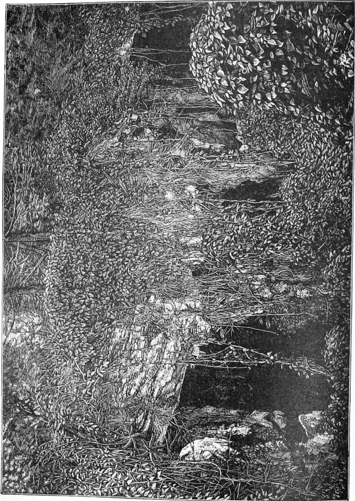
FIG. 18.—Entrance to the Convolvulus Cave, Walsingham, Bermudas. (From a photograph.)
