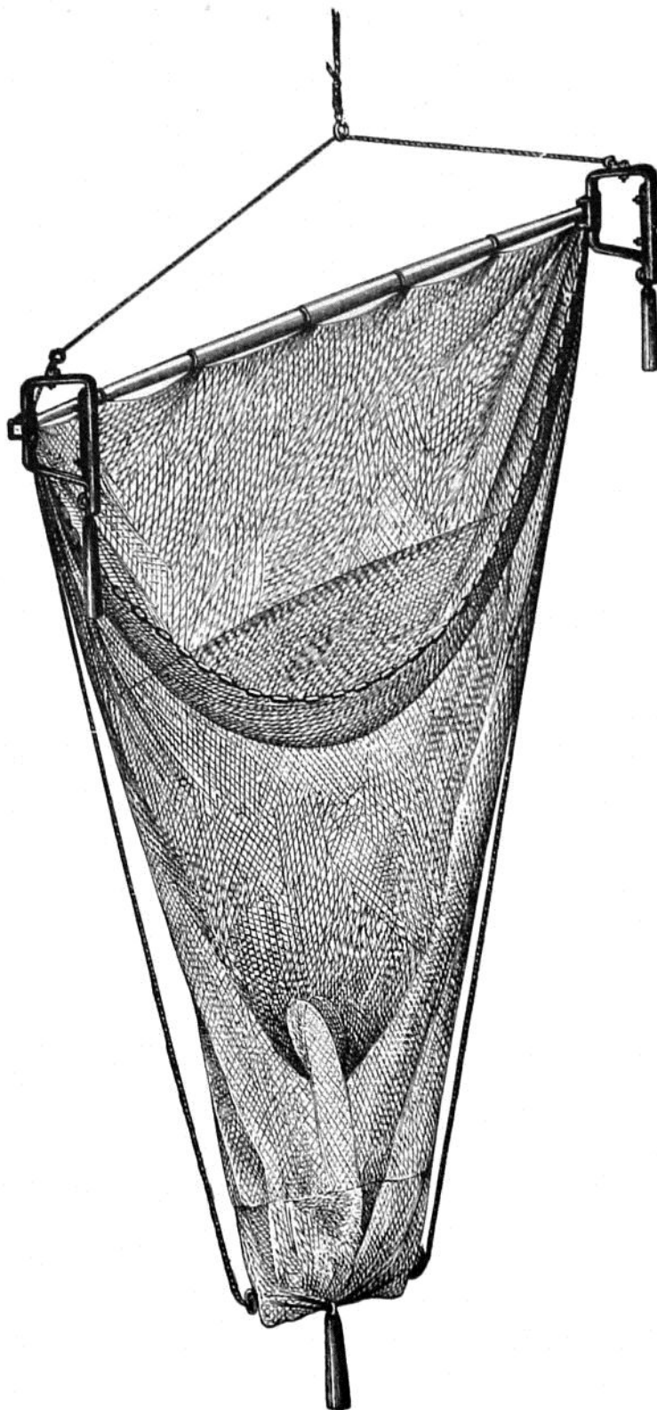
FIG. 18.—The Deep-sea Trawl.
