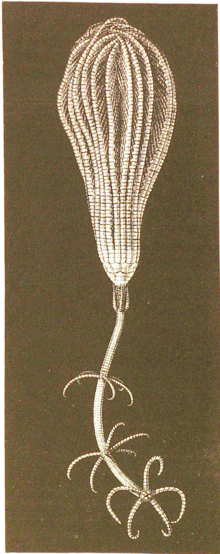
FIG. 71.— Pentacrinus wyville-thomsoni , JEFFREYS. Natural size. (No. 17, 1870.)
