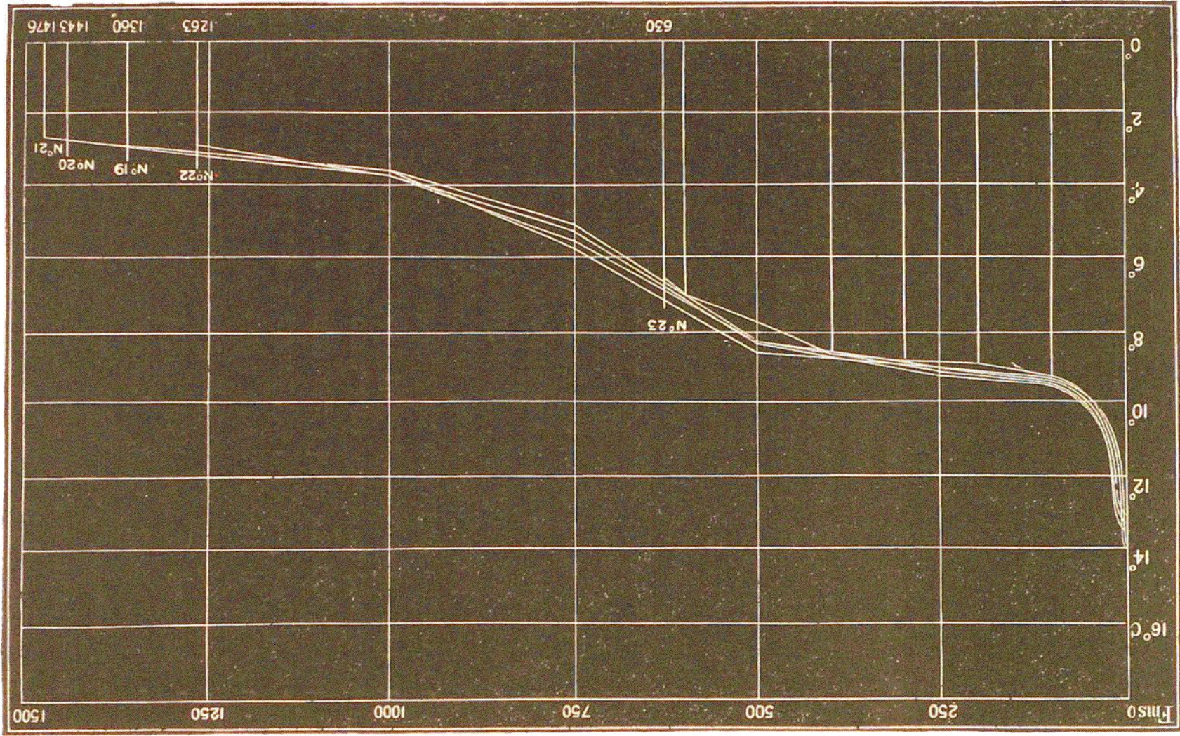
Fig. 58.—Curves constructed from serial and bottom soundings in the channel between Scotland and Rockall.
