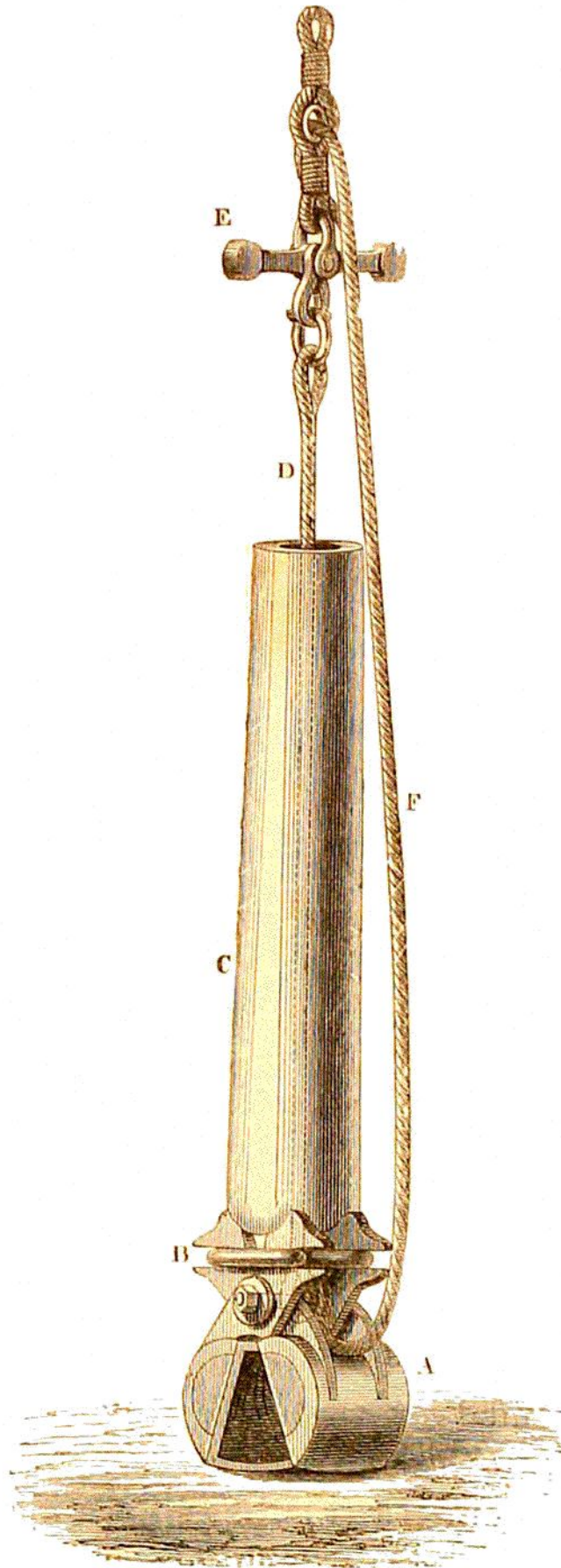
FIG. 40. — The 'Bull-dog' Sounding Machine.
