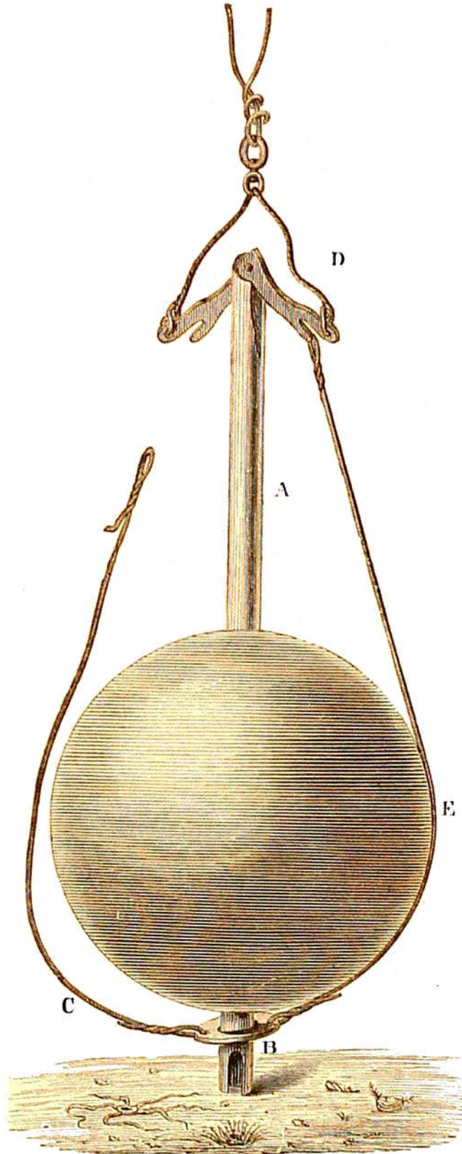
FIG. 39.—Brooke's Deep-Sea Sounding Apparatus.
